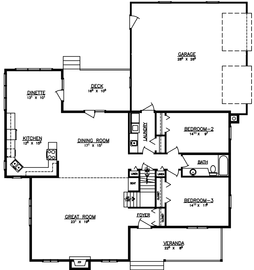
MAIN FLOOR AREA = 1772 S.F.
